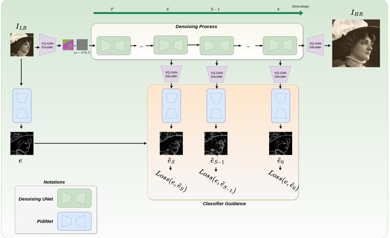
Figure 2. The overall pipeline of EdgeSR: For the first step is generated latent representation of LR image. In reverse process, starting from S step z_s is decoded into spatial image using a VQ-GAN decoder. PiDiNet architecture is then applied to image for edge detection, outputting a predicted edge map \tilde{e} . The loss L(\tilde{e}, e) = \|\tilde{e} - e\|^2 quantifies the discrepancy between the predicted and ground truth edge maps. Following this, the anti-gradient is computed to adjust the latent representation serving as the initial state for the subsequent denoising phase in the diffusion process.
